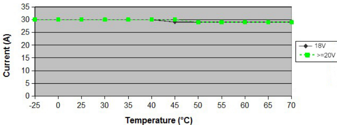
Maximum current at 12V output [18V,32V]
